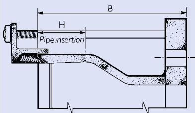
Expanded sleeve
