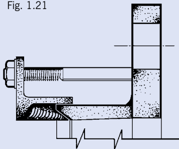
Straight sleeve
