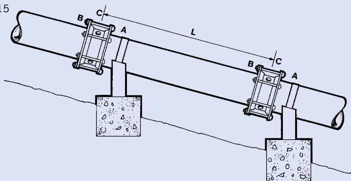
Typical support of inclined pipelines.
