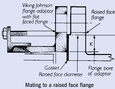
Mating to a raised face flange
